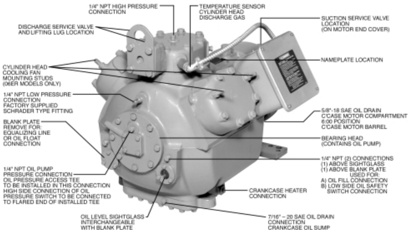
Figure 2 06E 6-Cylinder Compressor 65, 75, 99 Cfm (1.84, 2.12, 2.80 m 3 /m)
