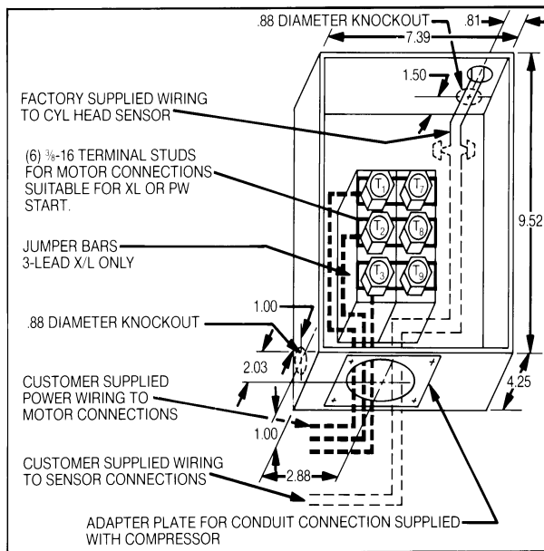
Figure A Terminal Box Arrangement
