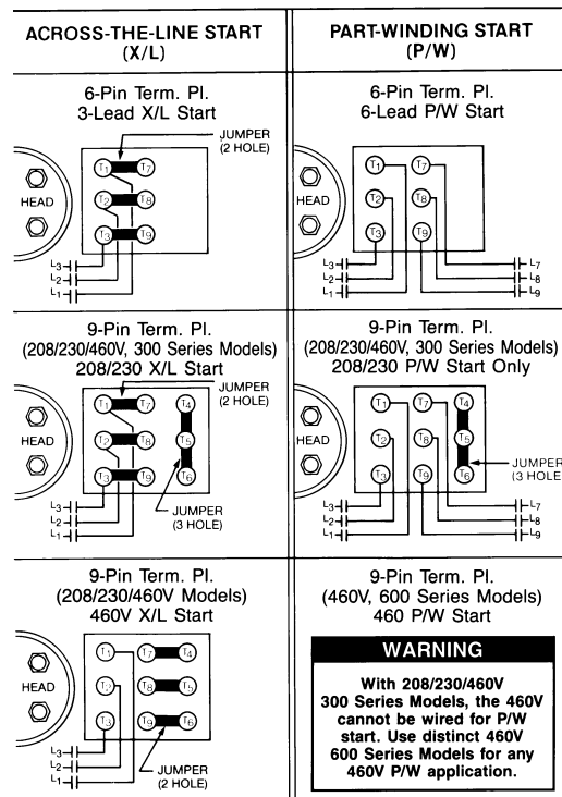
Figure 3 Terminal Plate Wiring
